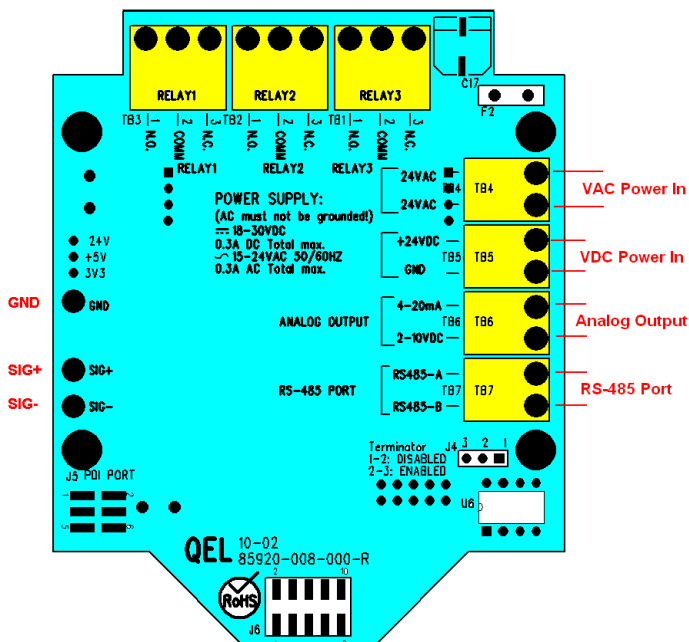
Q5 Terminals
